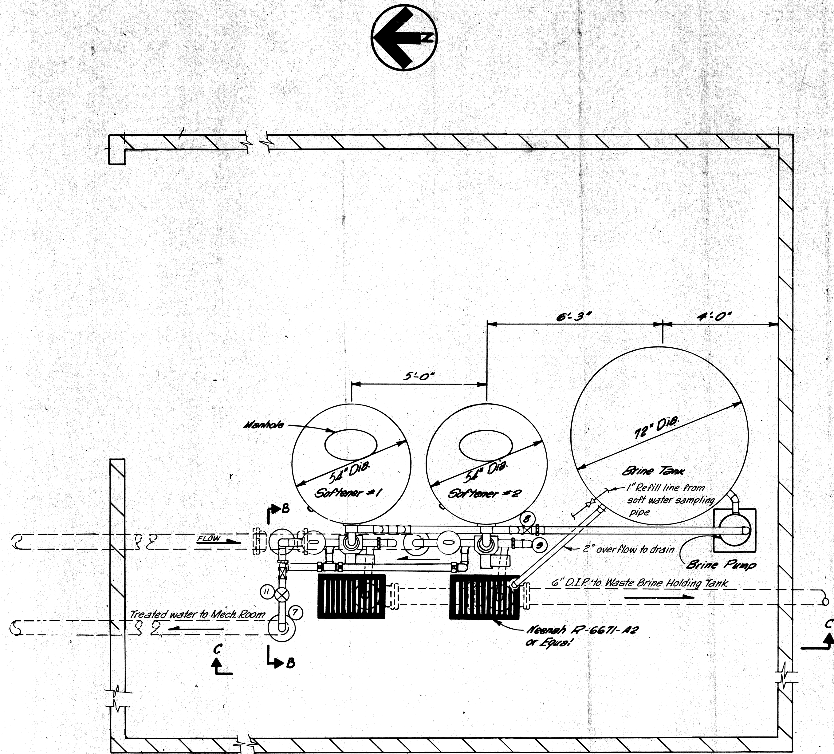
PLAN Scale 1/8" = 1'-0"
