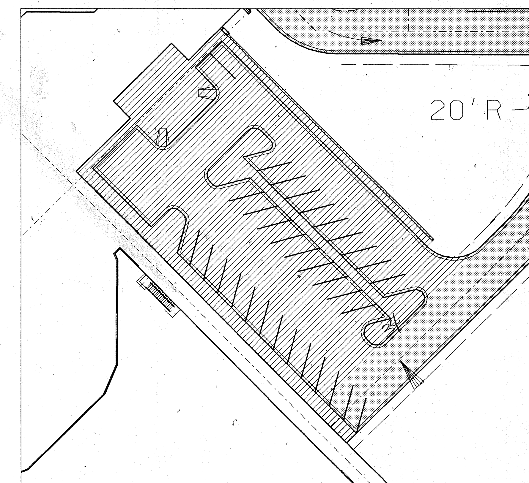
3 C-13 CRIME LAB AREA PARKING AND LAYOUT
