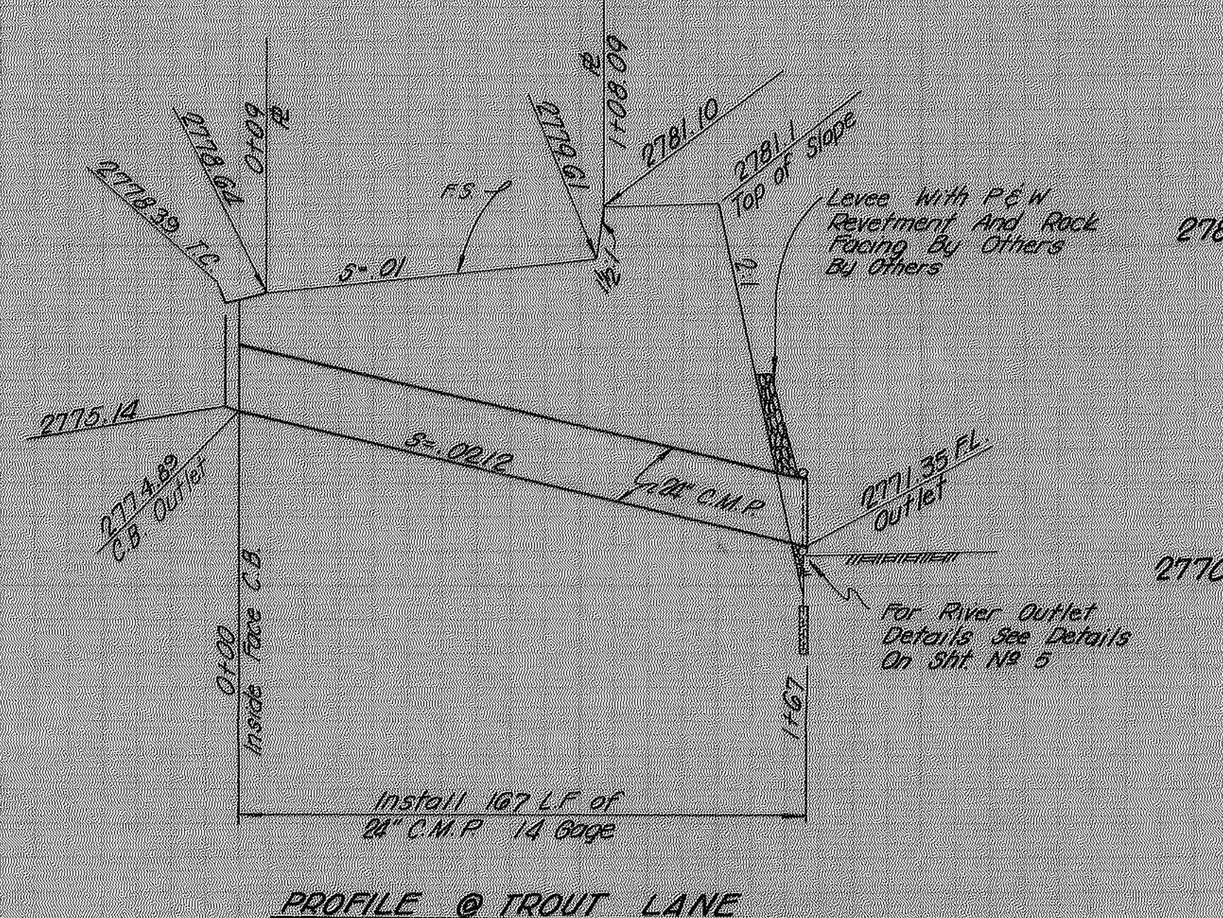
PROFILE @ TROUT LANE
