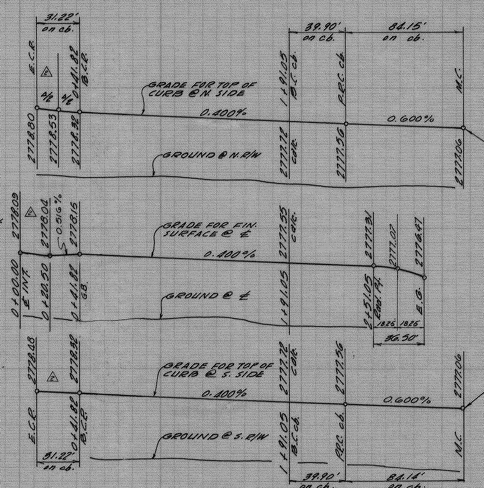
PROFILE SCALES HORIZ. 1"=40' VERT. 1"=4'
