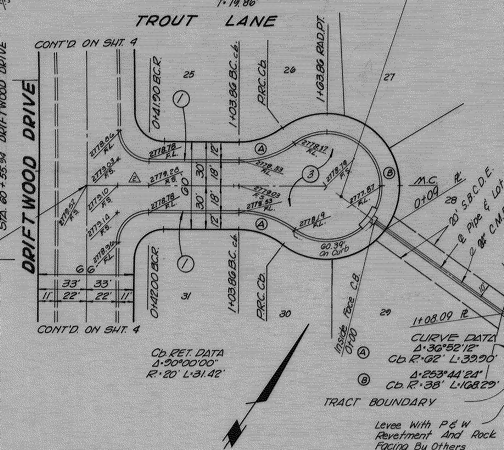
PLAN: Scale: 1"=40'
