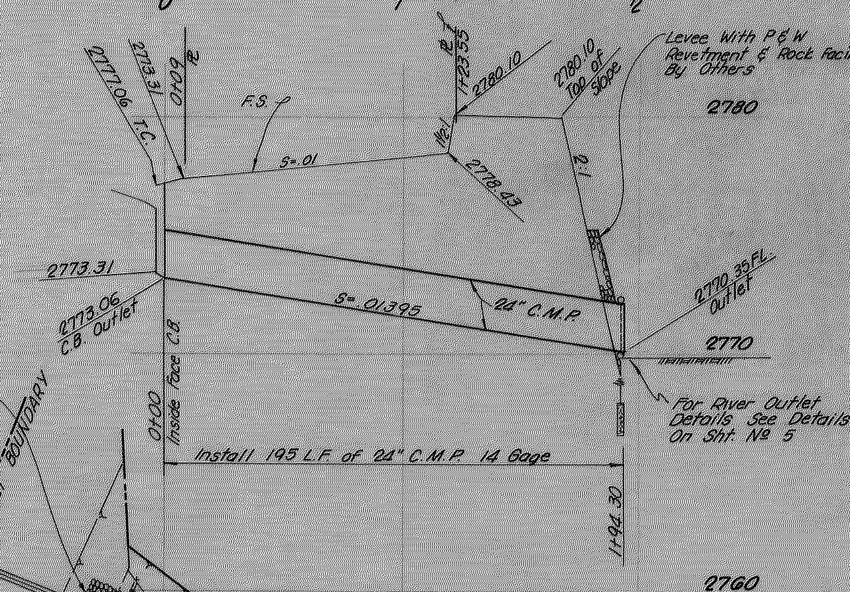
PROFILE AT TARPON LANE
