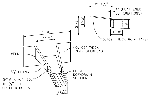
TAPERED INLET
