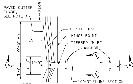
NOTE A In sag location, use 10'-0" length of paved gutter flare on both sides of inlet. PLAN
