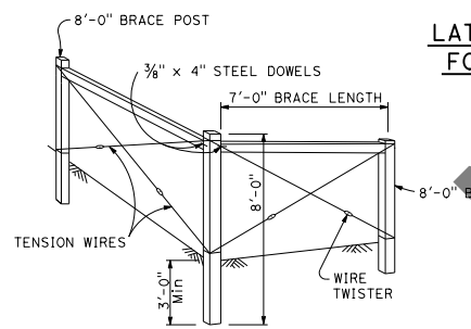
END AND CORNER POST ASSEMBLY
