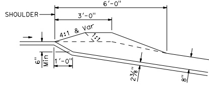
SECTION G-G
