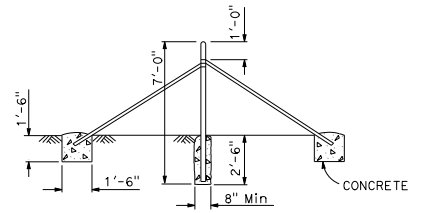
PULL POST ASSEMBLY
