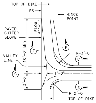
PLAN MOUNTABLE DIKE
