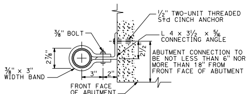
ABUTMENT CONNECTION
