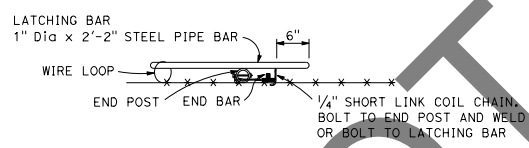
LATCHING DEVICE FOR GATEWAYS See Note 1
