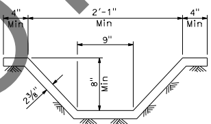
SECTION C-C See Note 1
