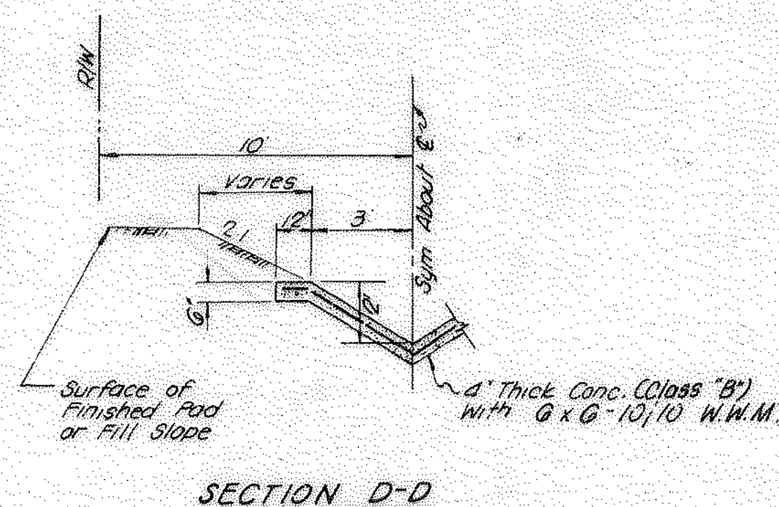
DETAILS OF INLET & DITCH NO SCALE
