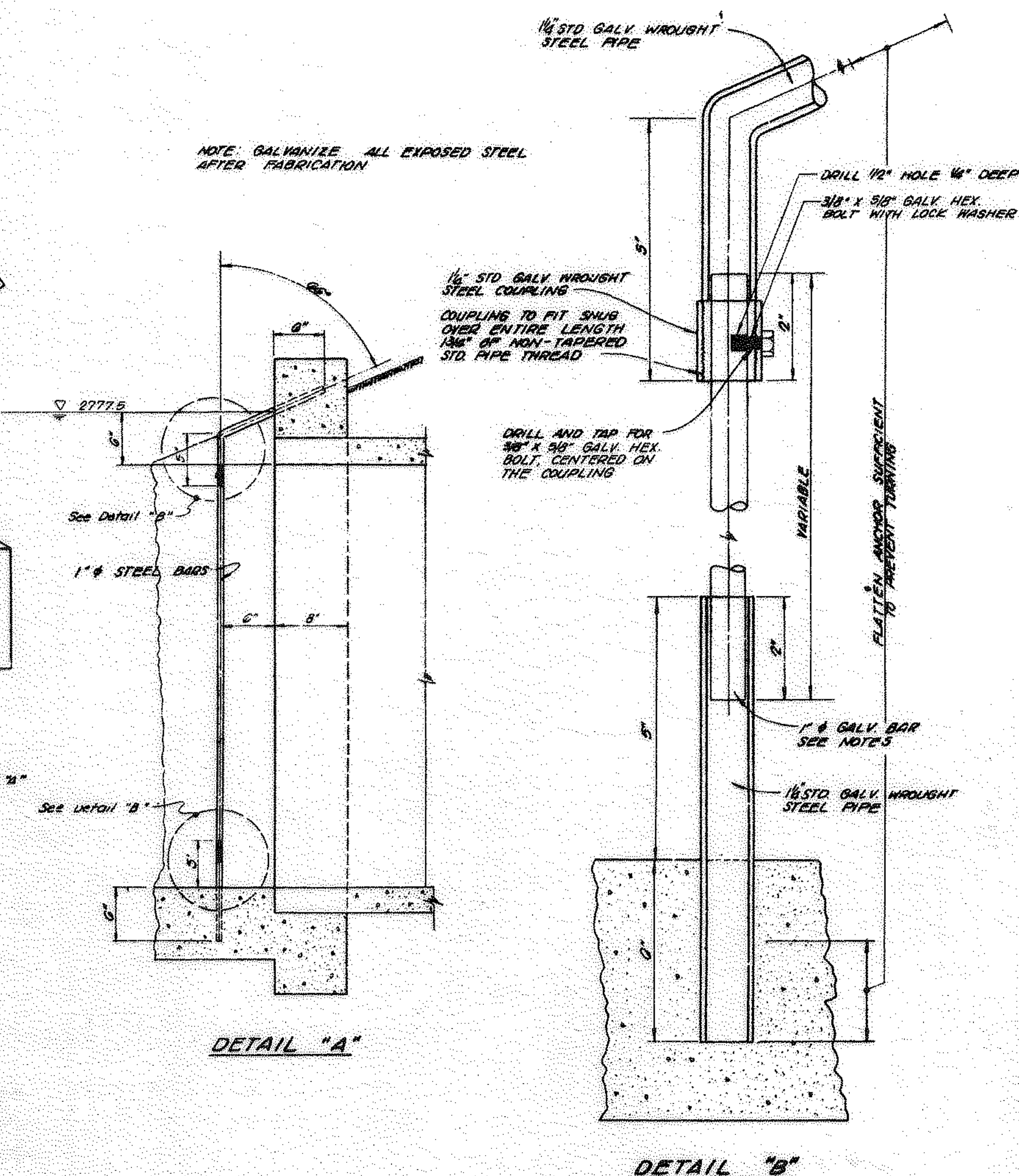
REMOVABLE PROTECTION BARS FOR OUTLET HEADWALL NO SCALE
