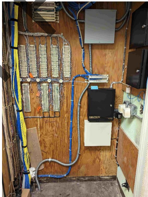
Detail 3/1 st - Telephone Closet on the First (1 st ) Floor
