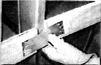
Overlap adjacent pieces when screwing into the framing.
