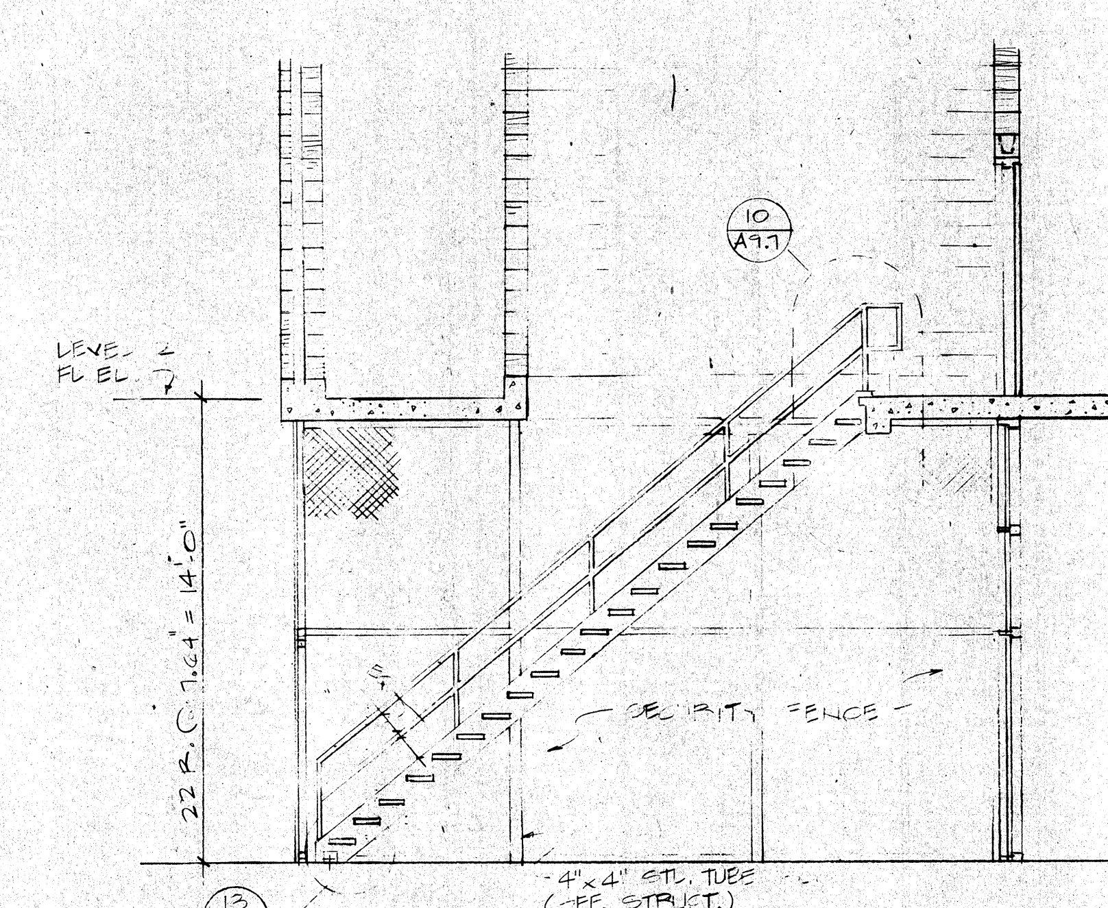
7 SECTION THRU STAIR
