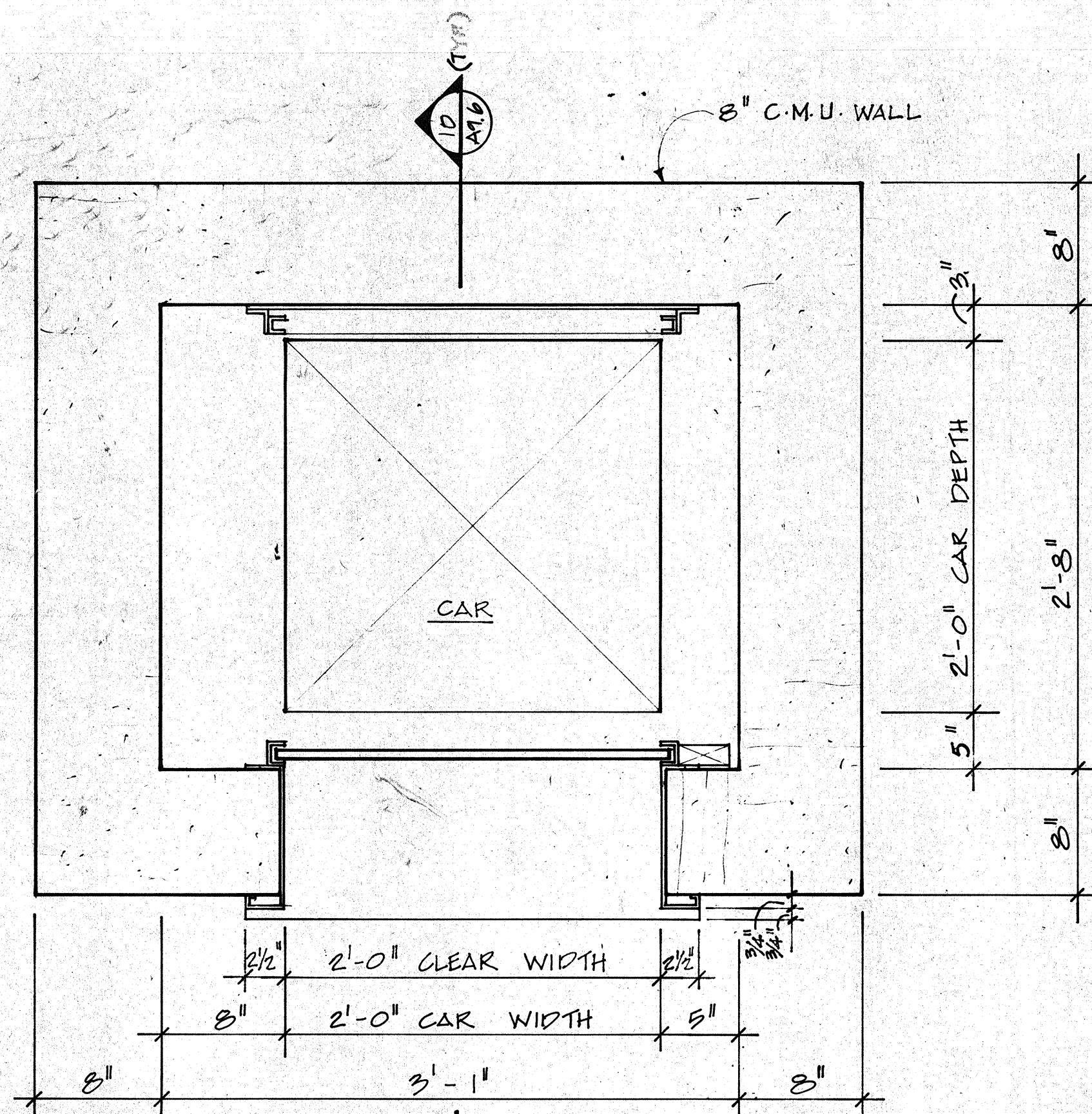
1 DUMBWATER PLAN SCALE: 1 1/2" = 1'-0"
