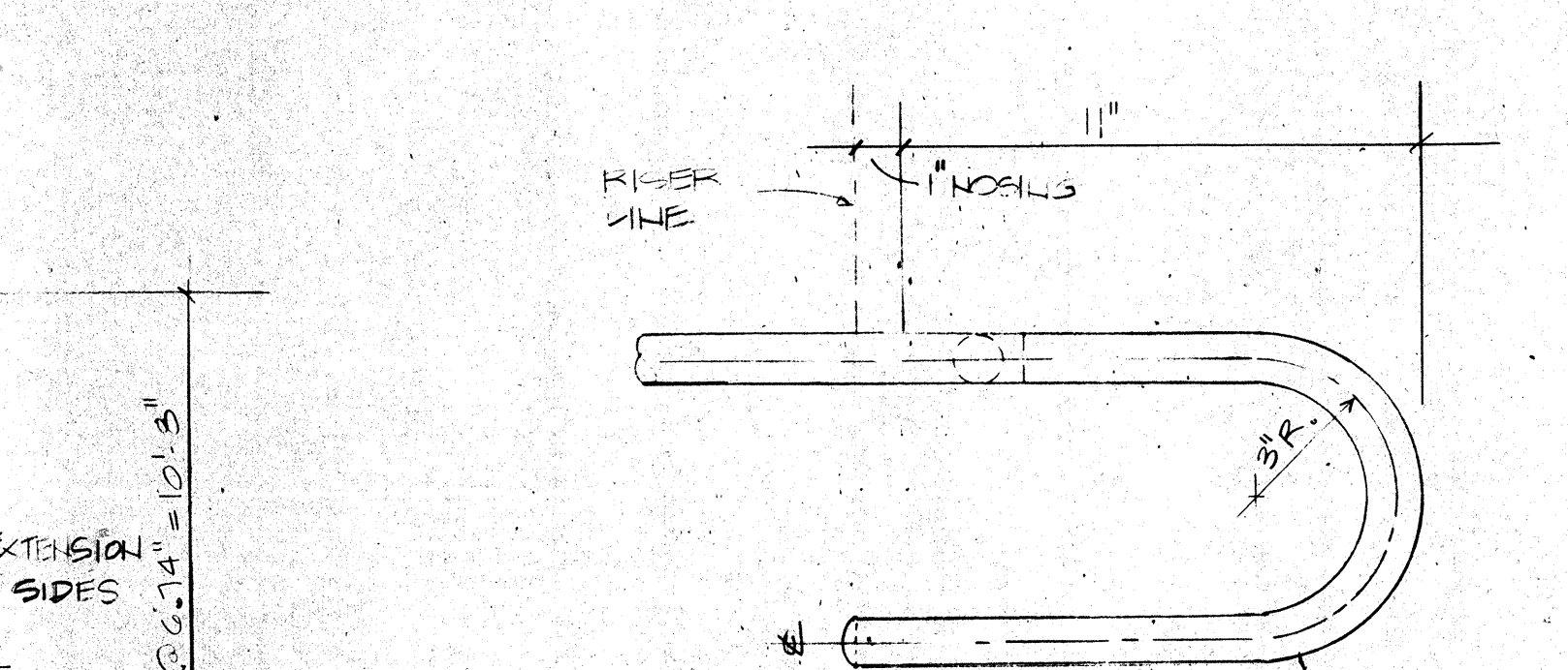
14 PLAN DETAIL - HANDRAIL
