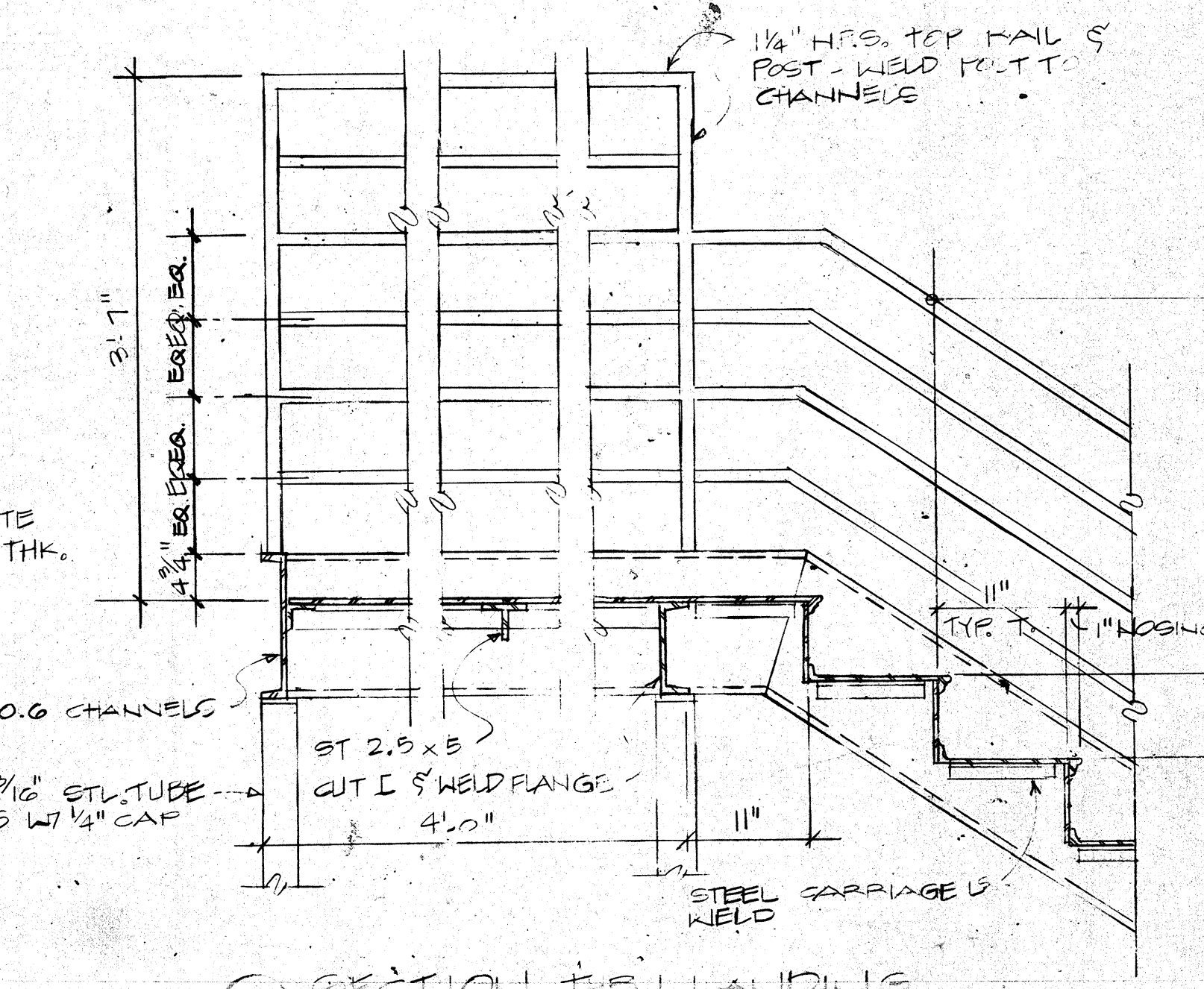
19 SECTION THRU LANDING
