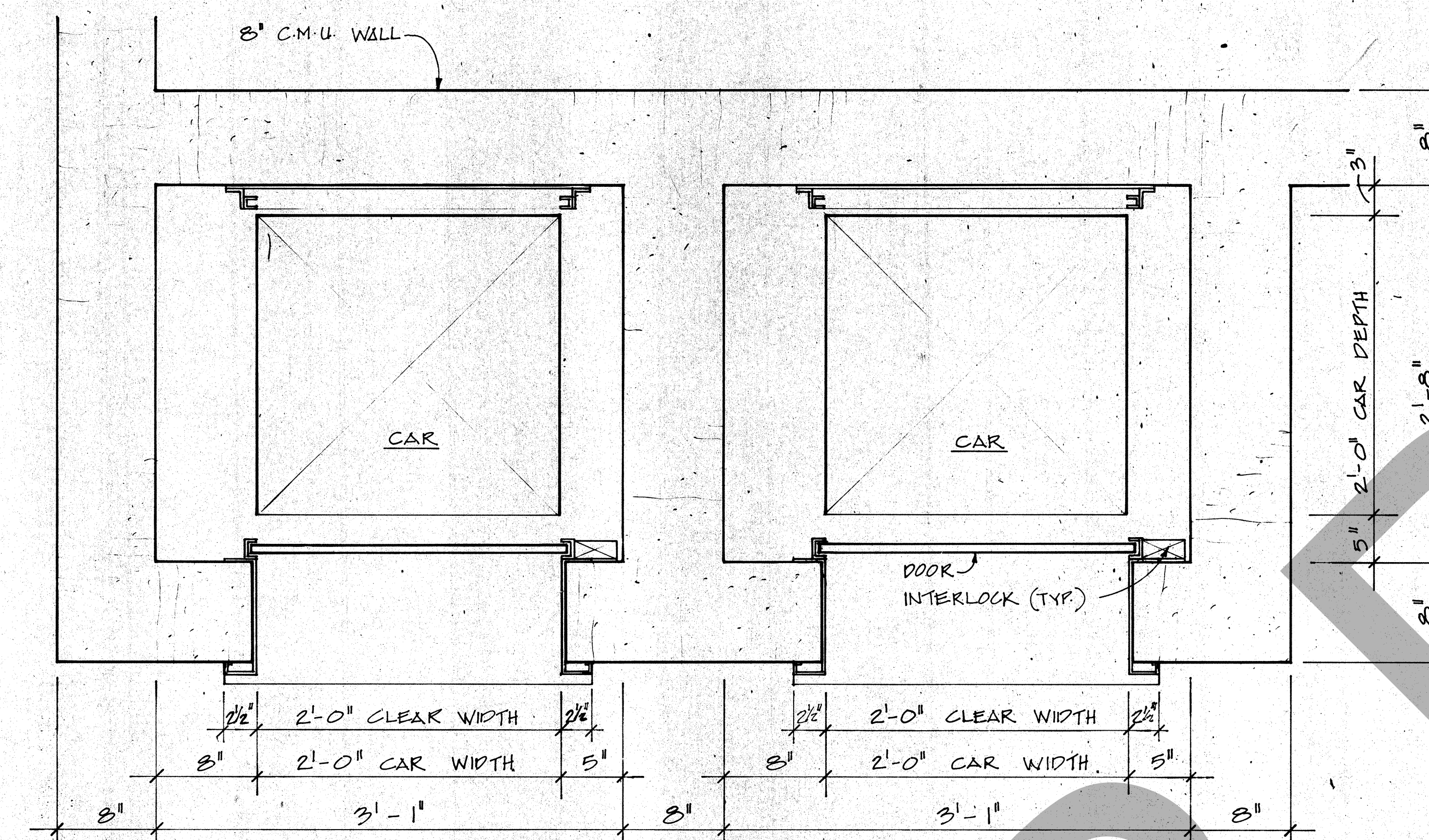
2 DUMBWATER PLAN SCALE: 1 1/2" = 1'-0"
