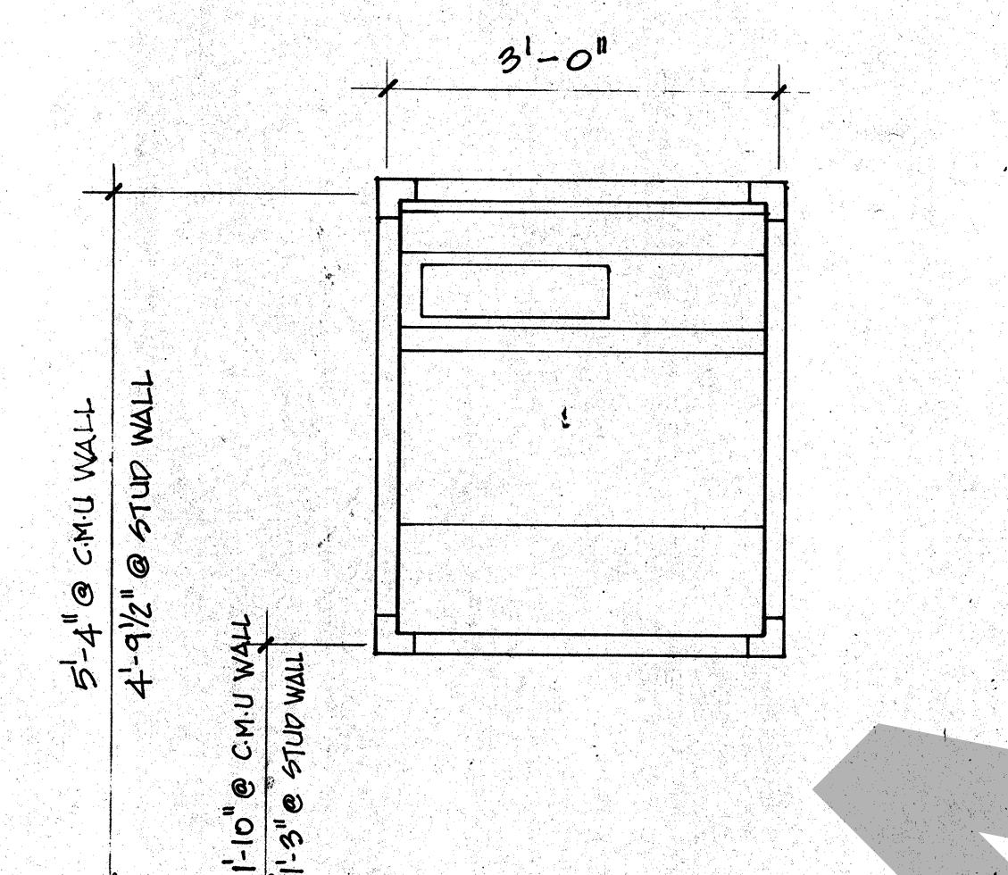
8 PNEUMATIC TUBE ELEVATION SCALE: 3/4" = 1'-0"
