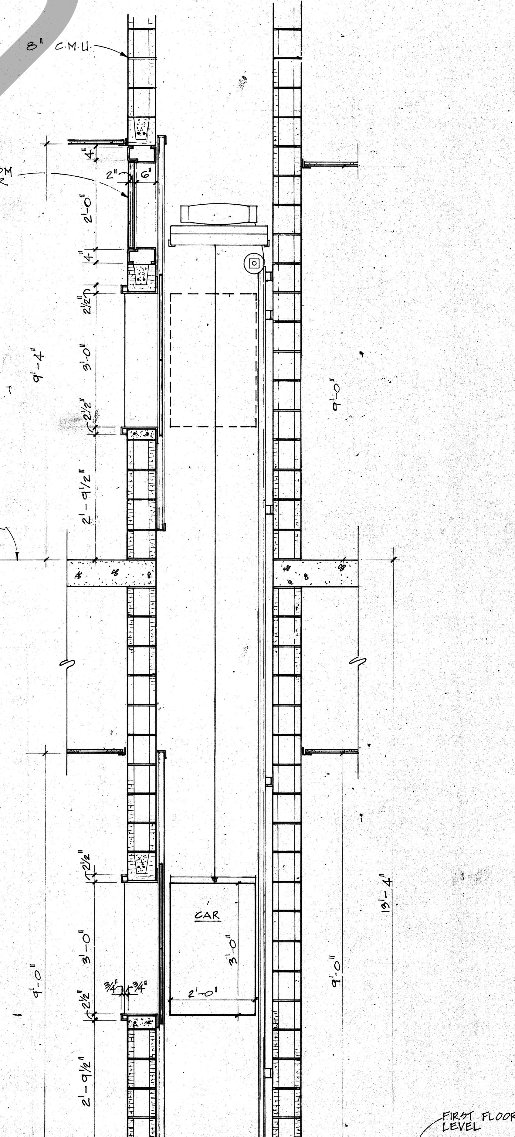
10 DUMBWATER SECTION SCALE: 3/4" = 1'-0"
