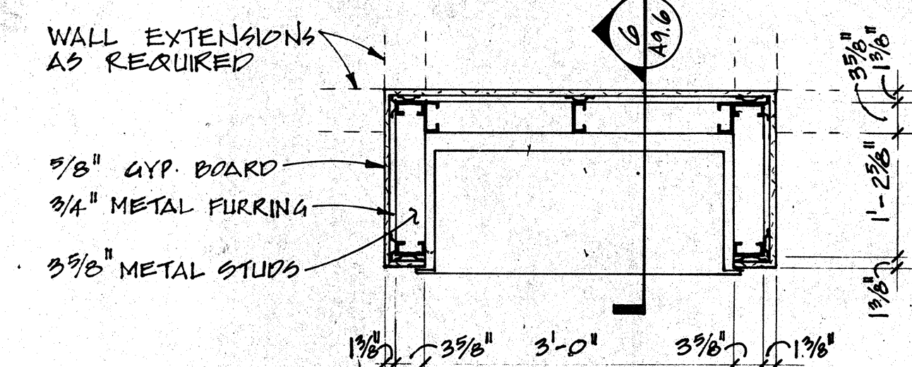
3 PNEUMATIC TUBE PLAN SCALE: 3/4" = 1'-0"
