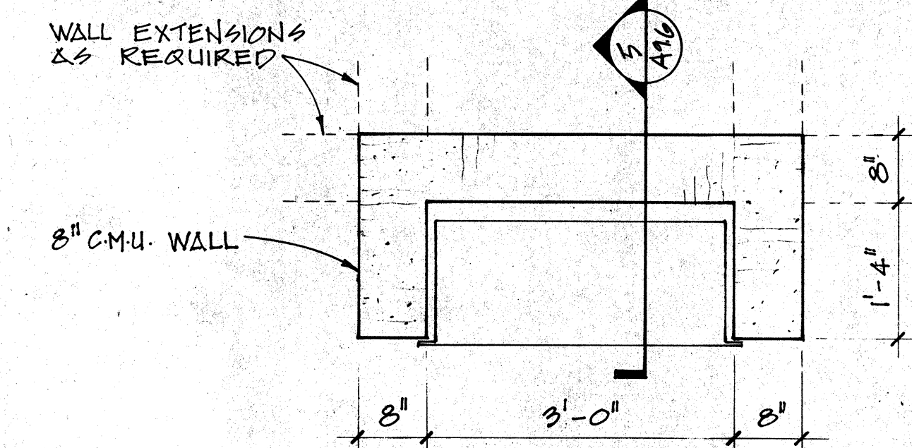
3 PNEUMATIC TUBE PLAN SCALE: 3/4" = 1'-0"
