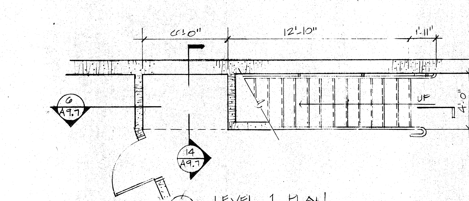
3 LEVEL 1 PLAN
