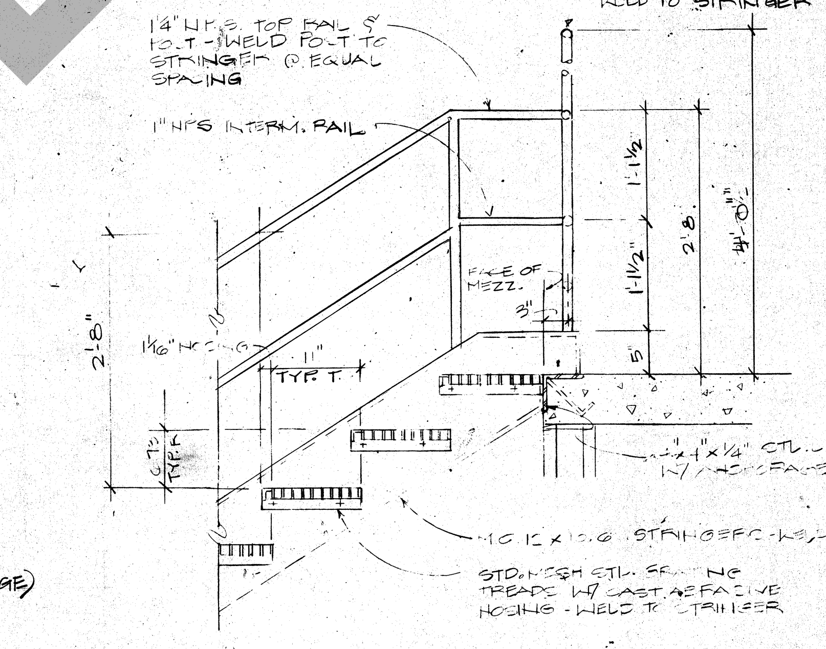
17 SECTION DETAIL @ LANDING
