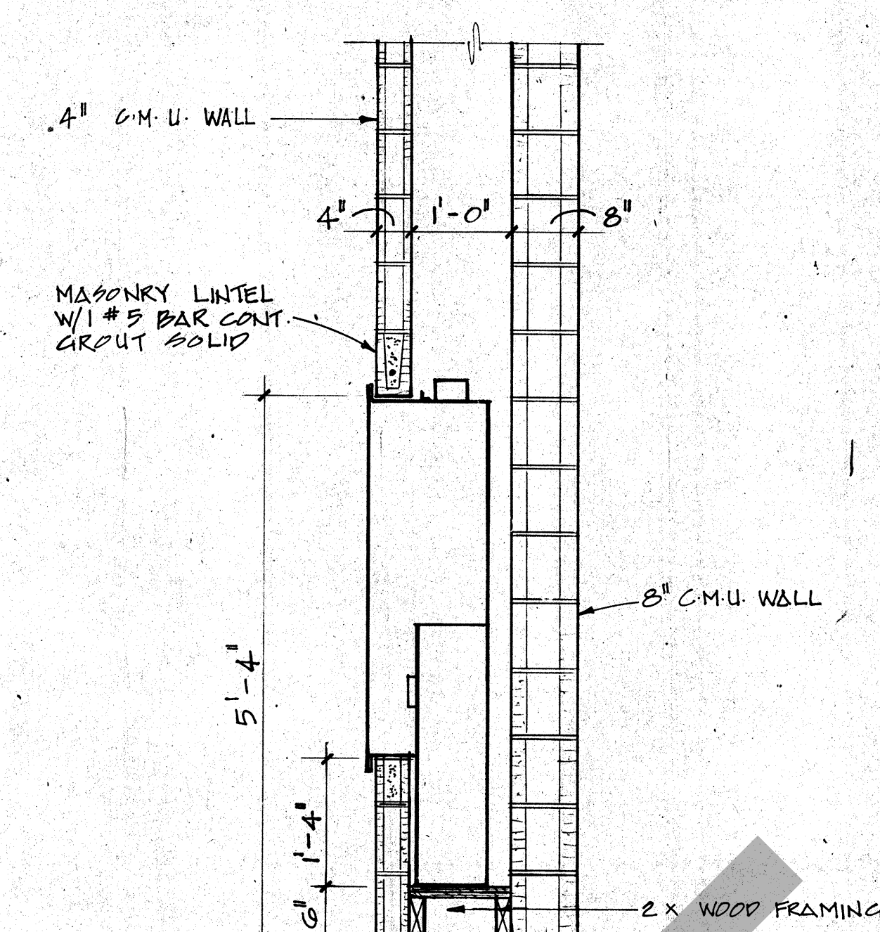
5 PNEUMATIC TUBE SECTION SCALE: 3/4" = 1'-0"
