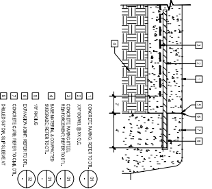
08 PAVING JOINT AT CURB
