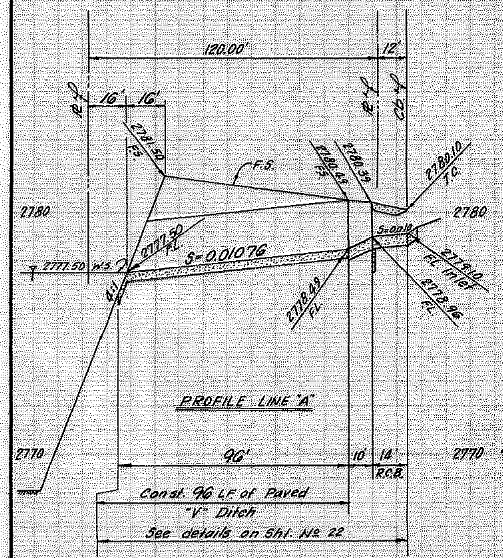
TYPICAL PROFILE OF INLET & DITCH NORTH & SOUTH Scale: Horiz. 1" = 40' Vert. 1" = 4'
