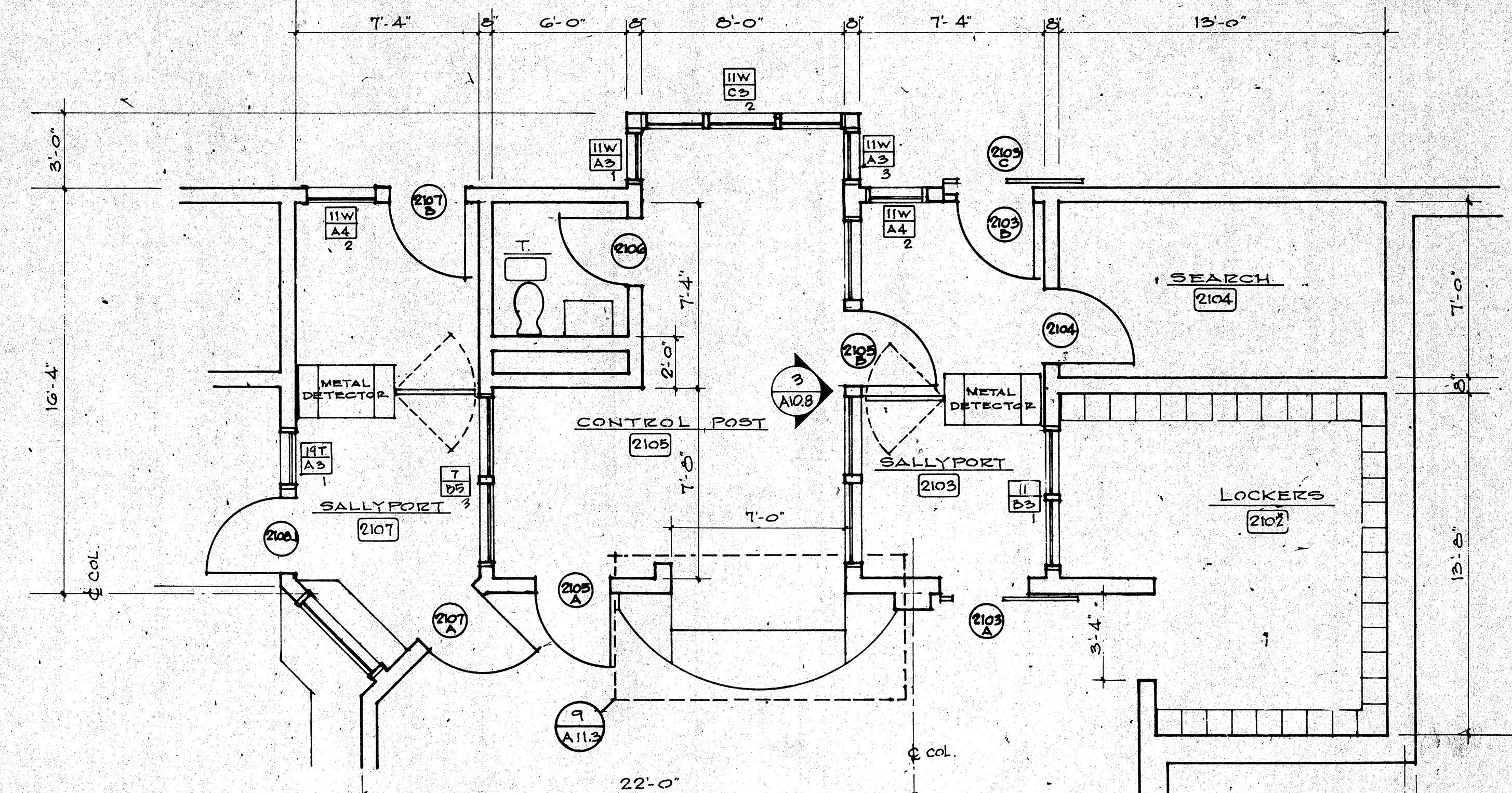
2 VISITING CONTROL ROOM SCALE: 1/4" = 1'-0"
