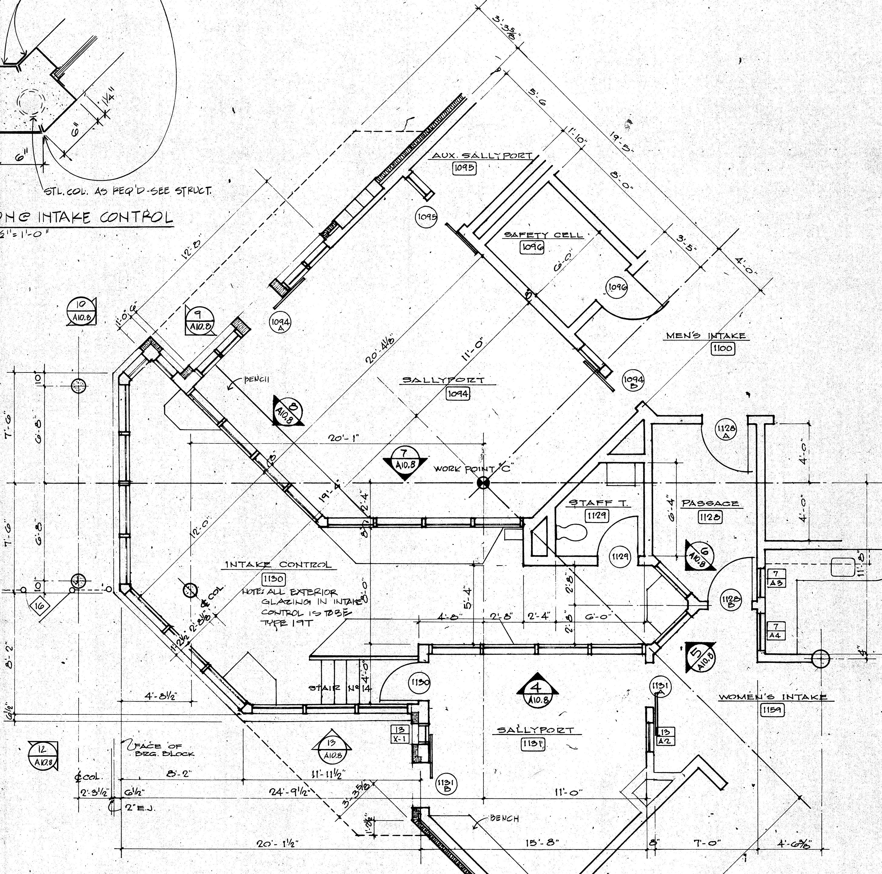
1 INTAKE CONTROL AREA SCALE: 1/4" = 1'-0"
