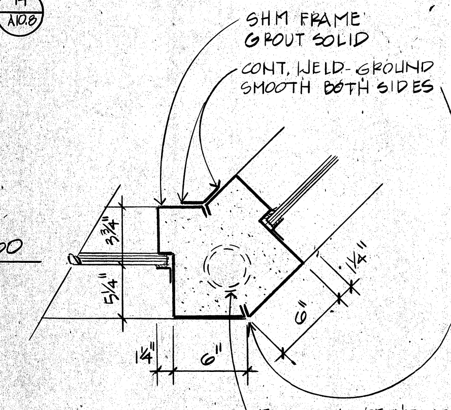
14 MULLION & INTAKE CONTROL SCALE: 1/2" = 1'-0"
