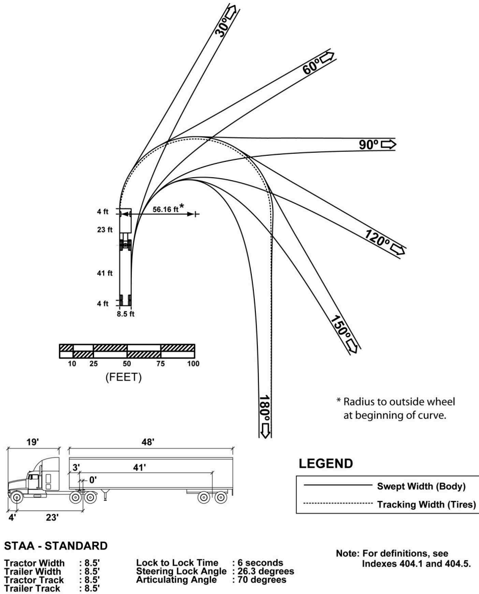
Figure 404.5A STAA Design Vehicle 56-Foot Radius
