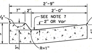
TYPE B4 CURBS
