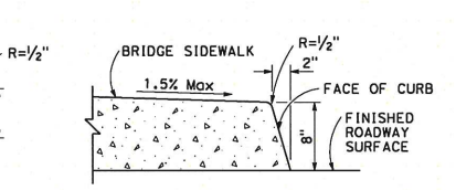
TYPE H CURB On Bridges
