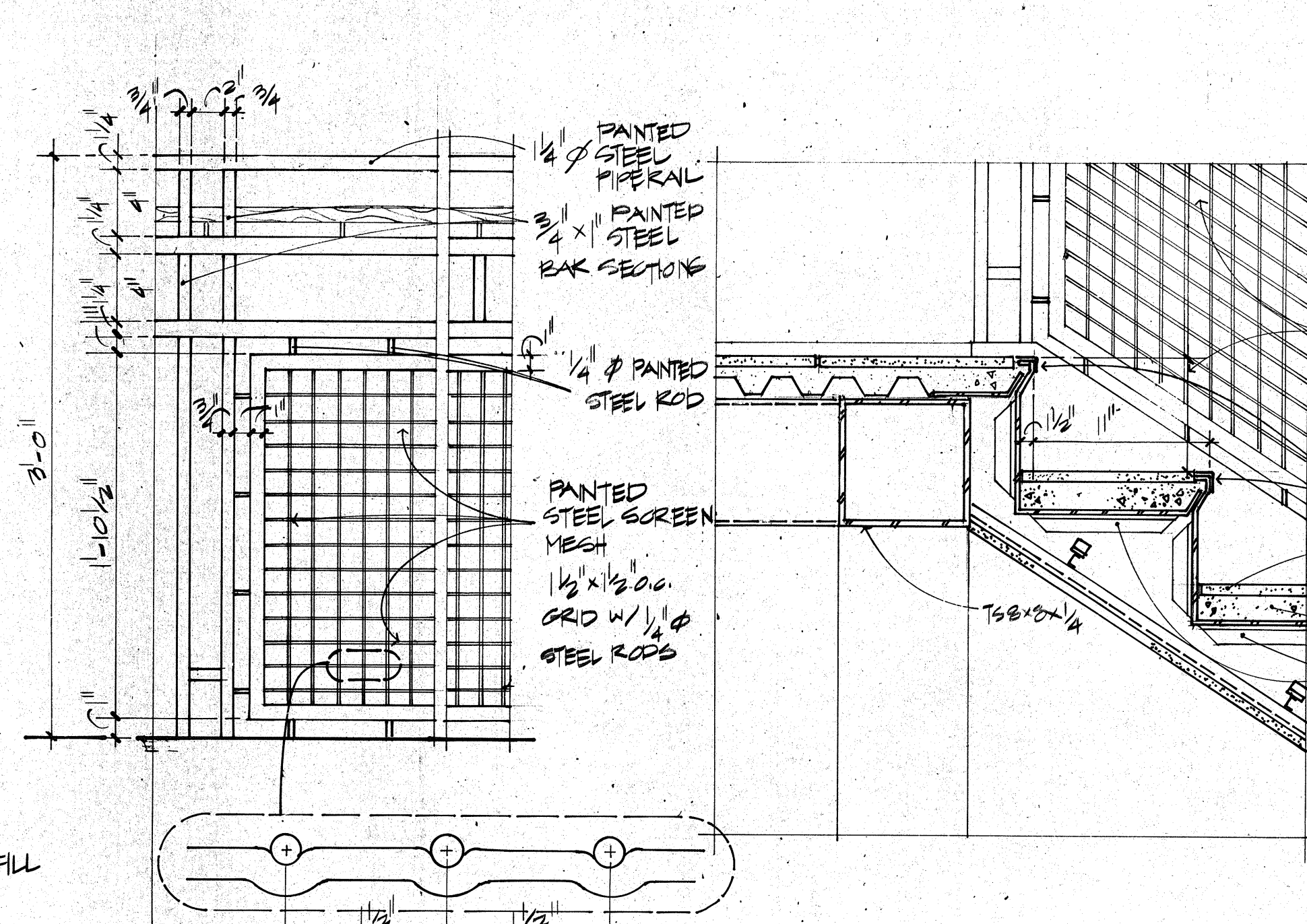
7 DETAIL @ STAIR TREAD
