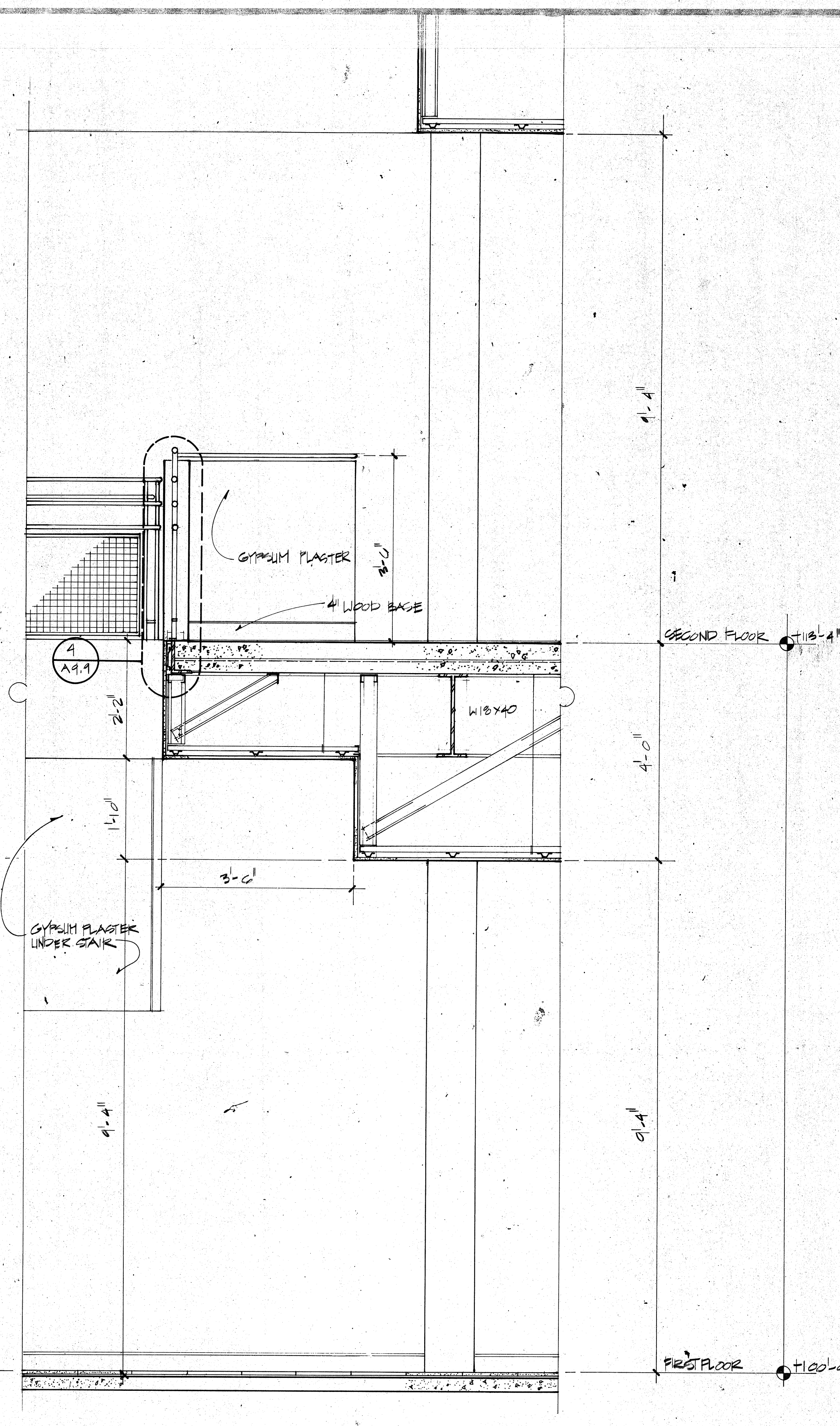
2 SECTION THRU BALCONY AND GUARDRAIL
