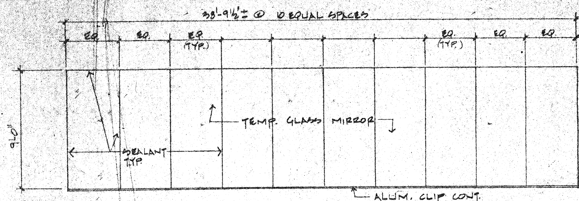
2 ELEVATION AT TRAINING RM. # 1013 SCALE: 1/4\"/>
