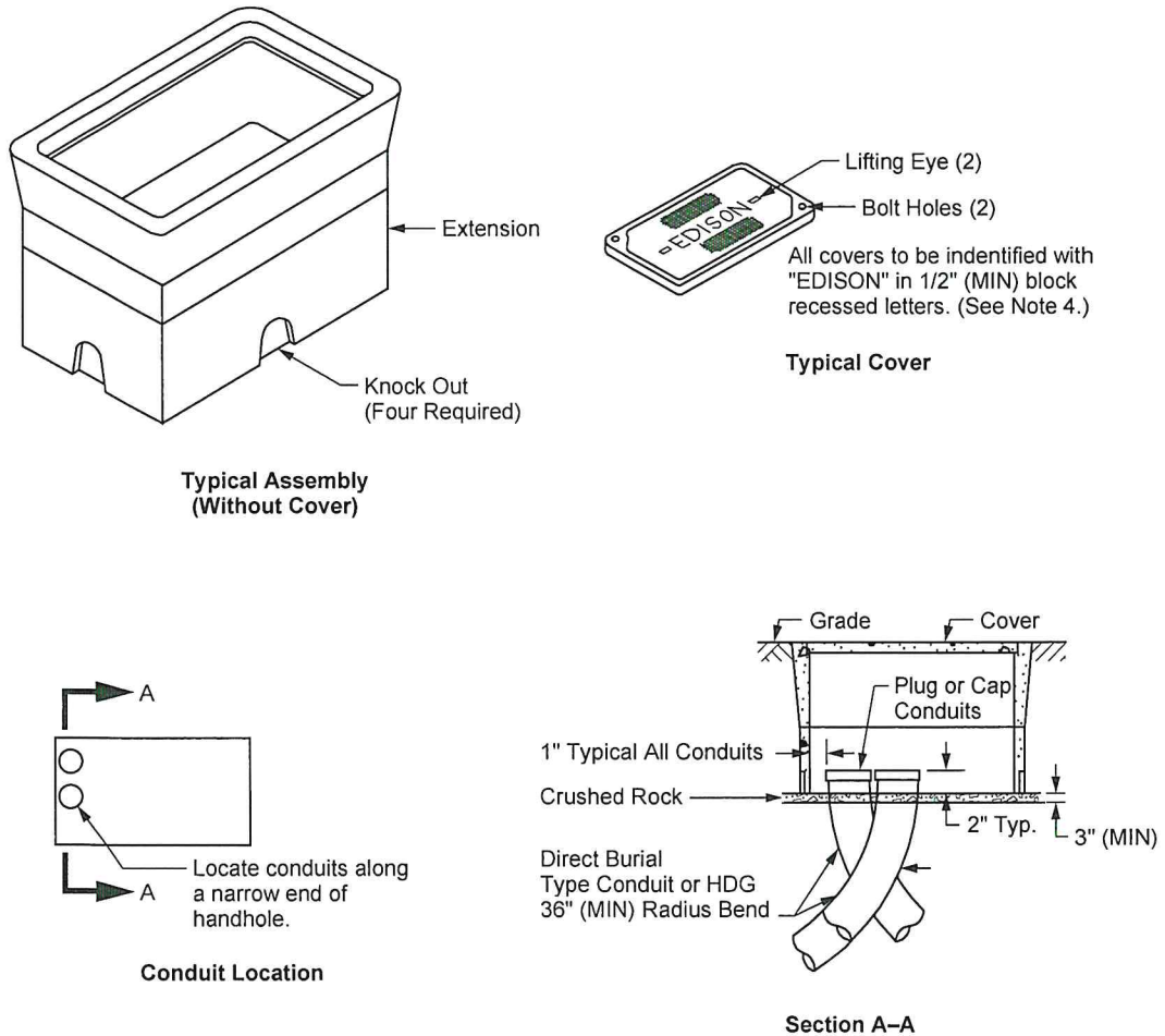
Figure HP 205-1: Typical Handhole Installation
