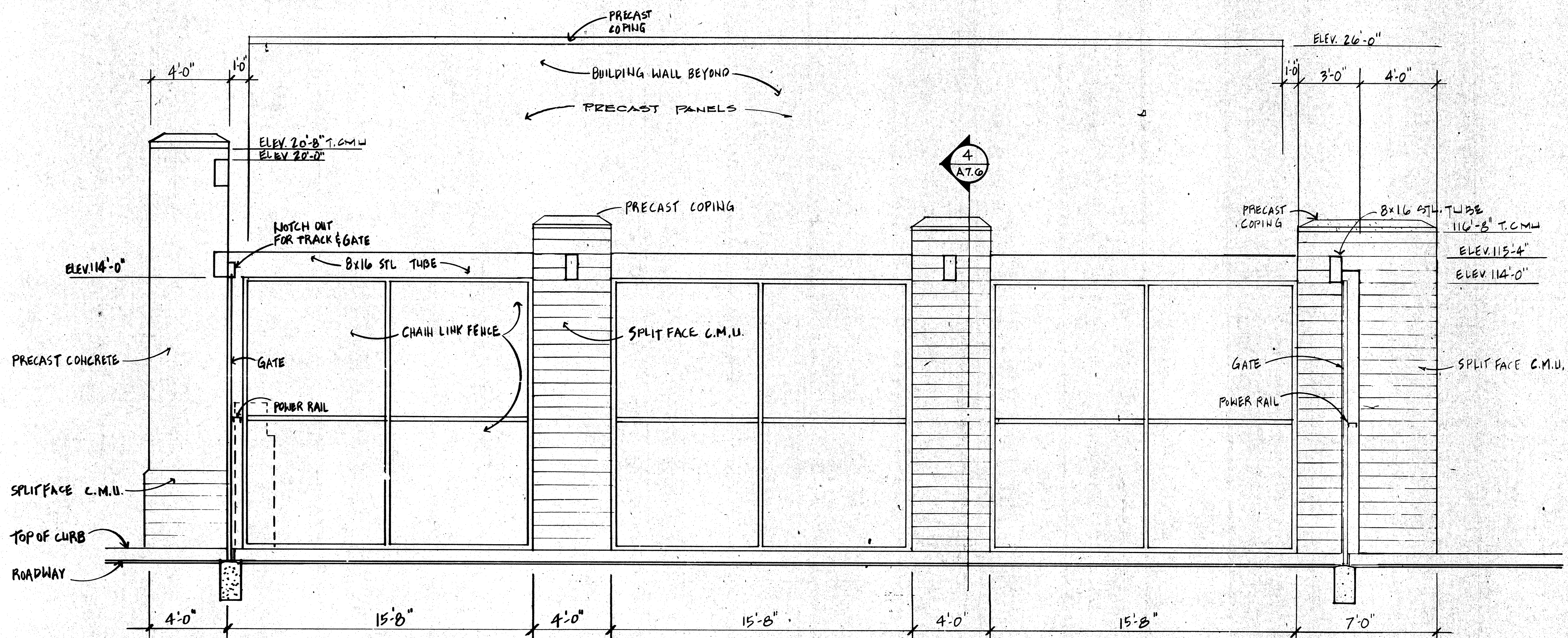
5 LONGITUDINAL SECTION - VEHICLE SALLYPORT SCALE 1/4" = 1'-0"
