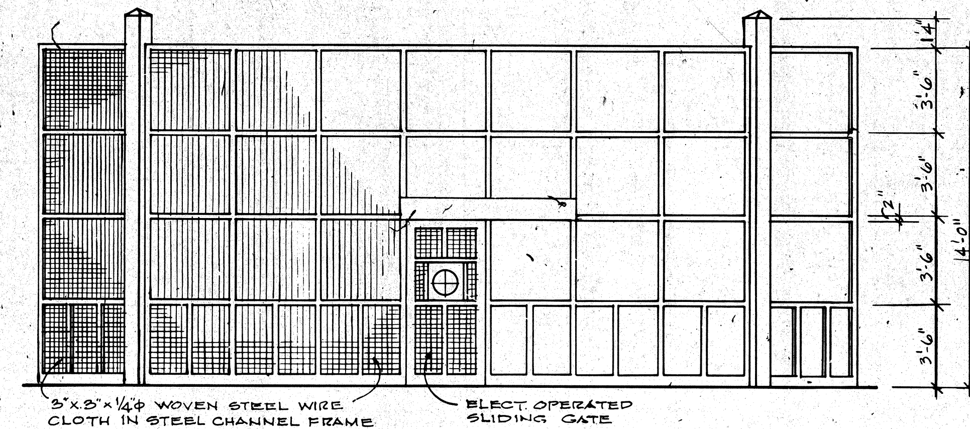
1 PEDESTRIAN SALLYPORT ENCLOSURE SCALE - 1/4" = 1'-0"
