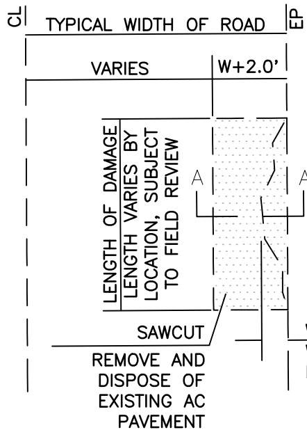
ROAD REPAIR PLAN NTS
