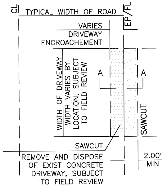
DRIVEWAY APPROACH DETAIL NTS
