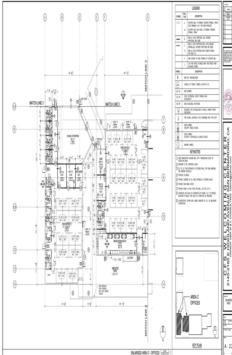
ENLARGED AREA C - OFFICES SCALE 1/8"=1'-0" 1
