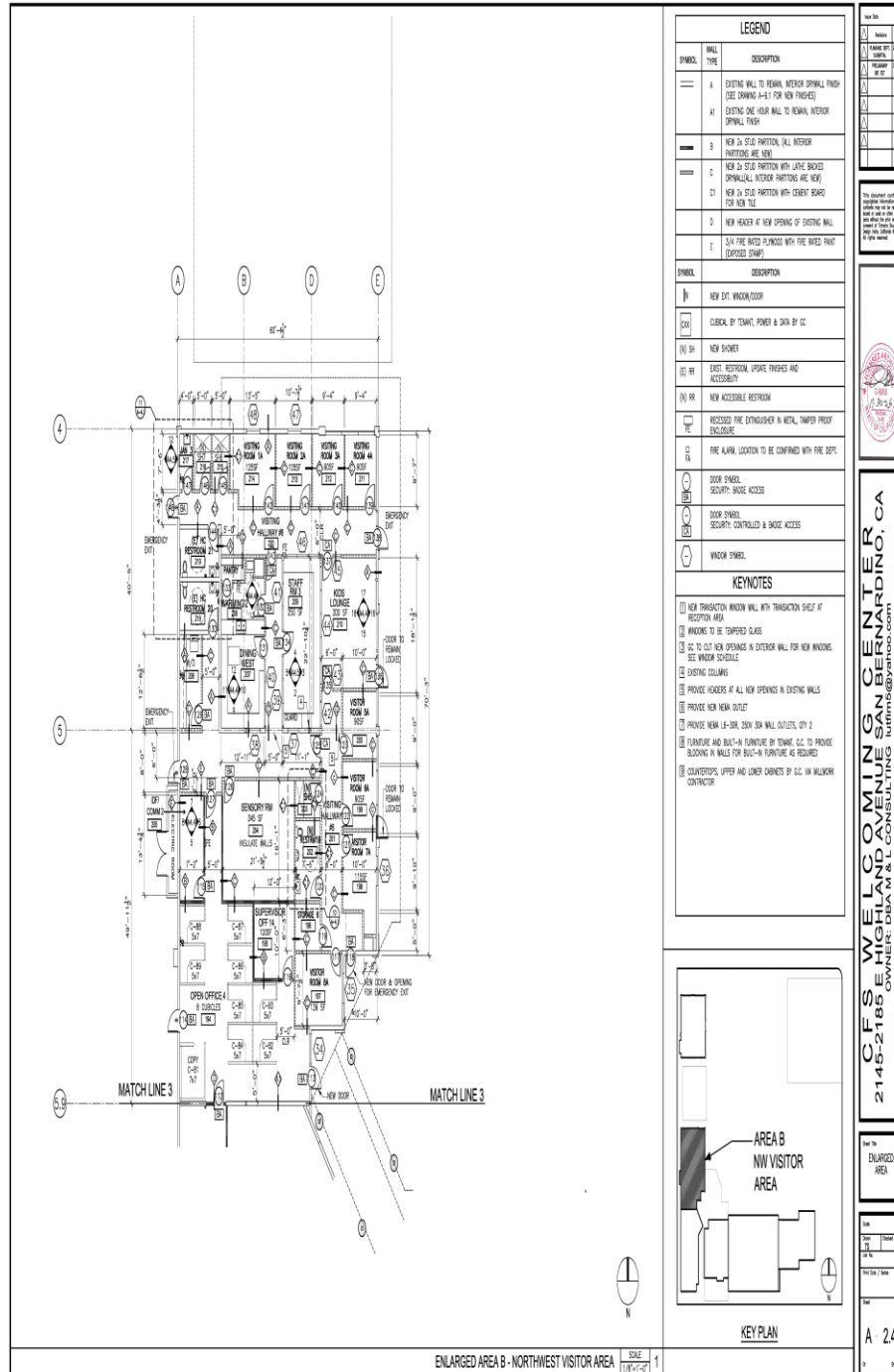
ENLARGED AREA B - NORTHWEST VISITOR AREA
