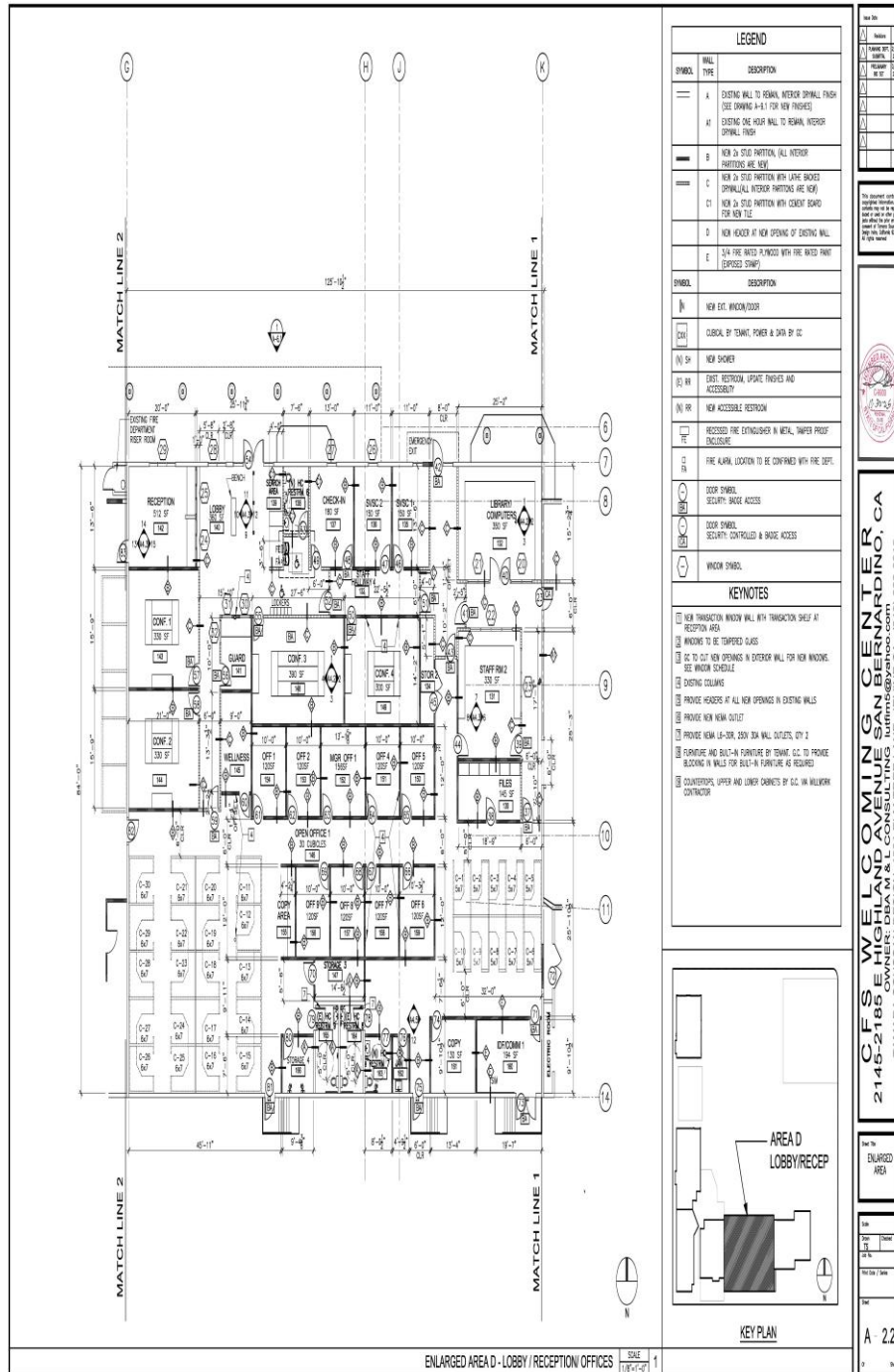
ENLARGED AREA D - LOBBY / RECEPTION OFFICES SCALE 1/8" = 1'-0" 1
