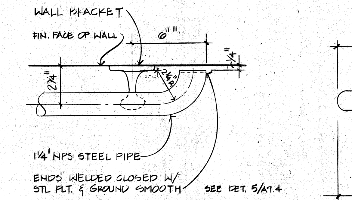
2 HANDRAIL RETURN PLAN VIEW SCALE: 3"=1'-0"
