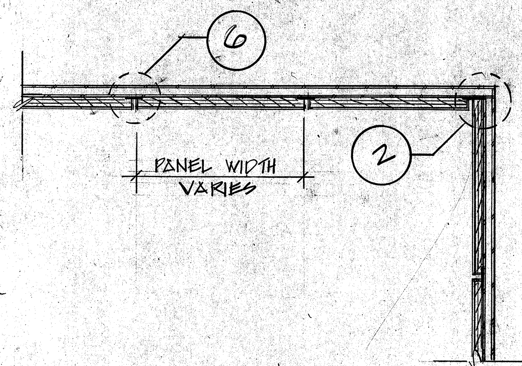
3 ELEVATOR CAR PANEL PARTIAL PLAN/SECTION SCALE: 1 1/2" = 1'-0"
