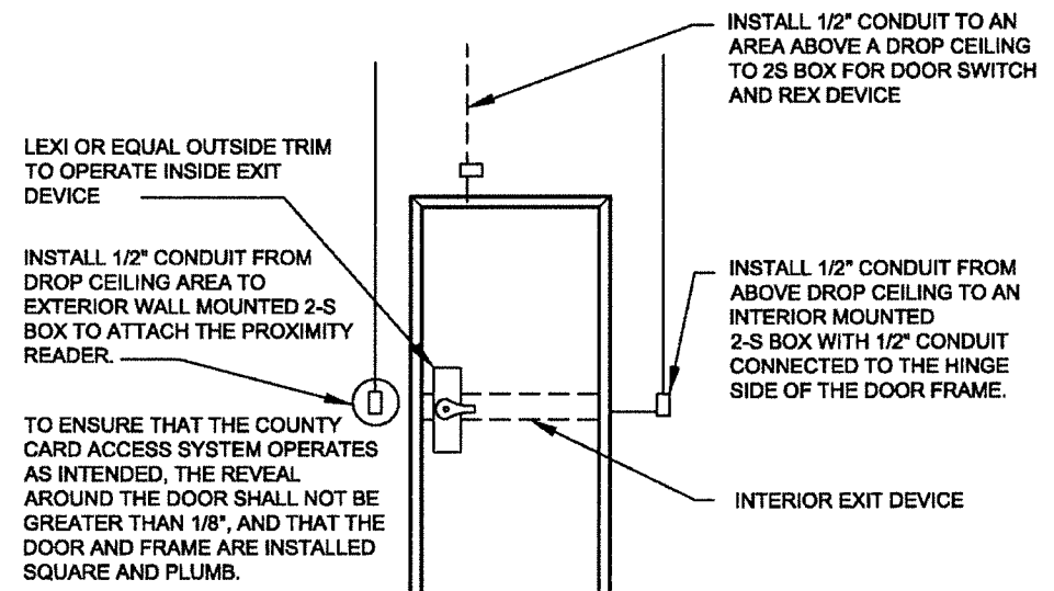
TYPICAL EXTERIOR CARD ACCESS DOOR
