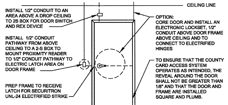
TYPICAL INTERIOR CARD ACCESS DOOR
