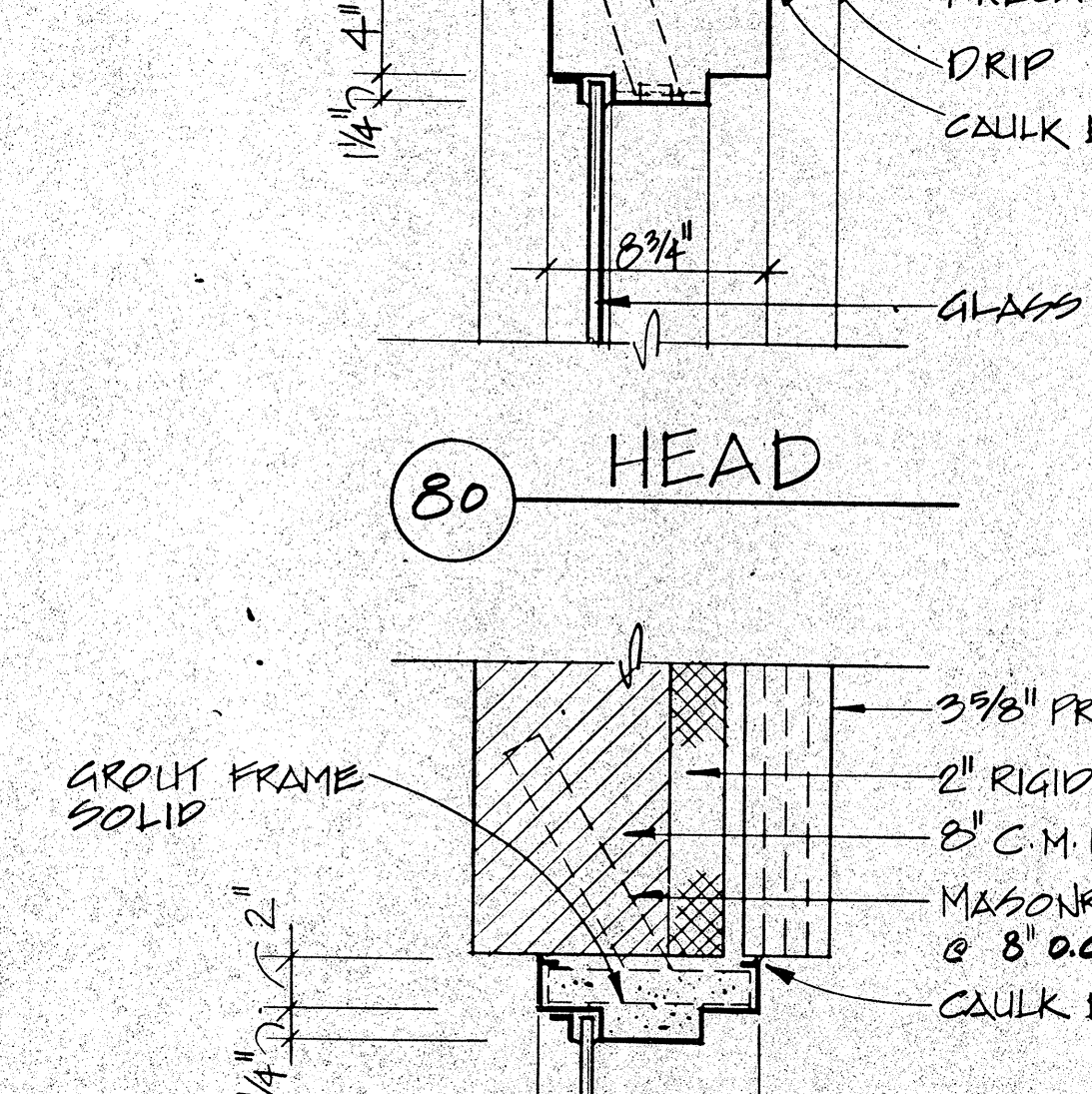
80 HEAD
