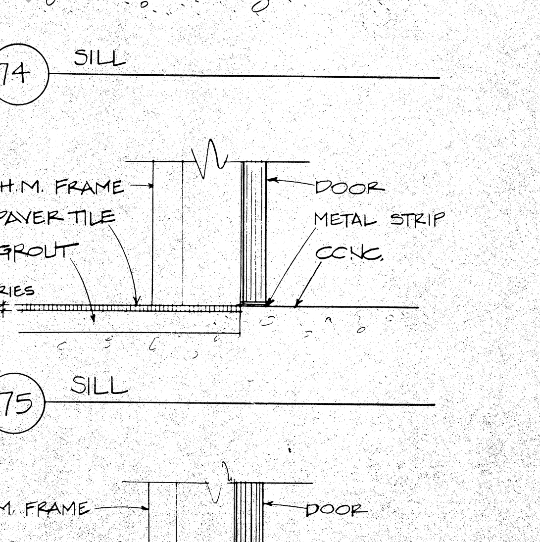
74 SILL
