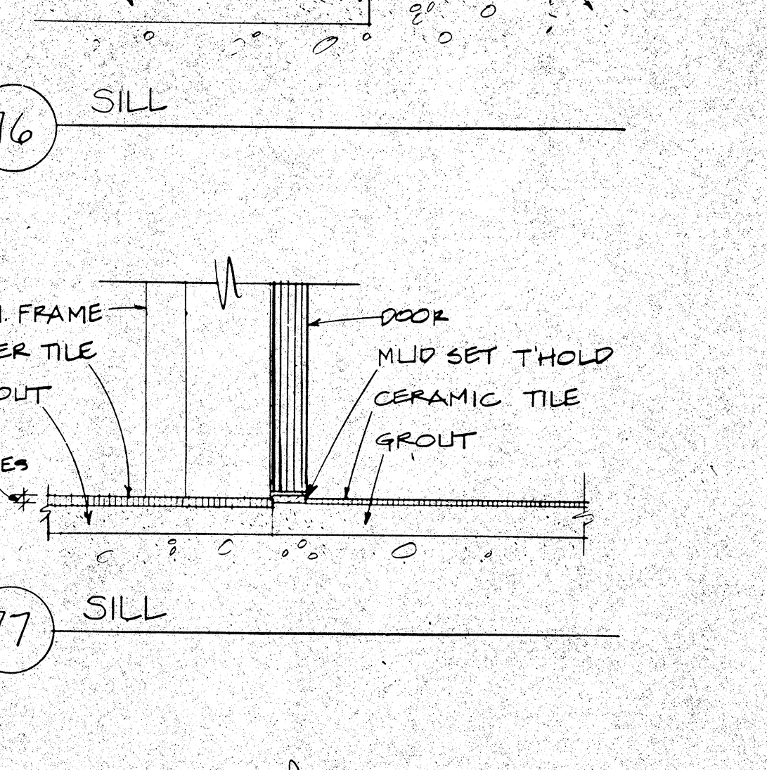
75 SILL
