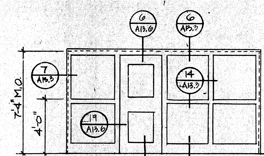
3 VISITING CONTROL POST 2105 (8 3/4") SCALE: 1/4" = 1'-0" UNO
