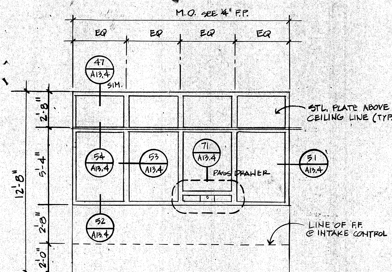
4 INTAKE CONTROL 1130 (15/8")
