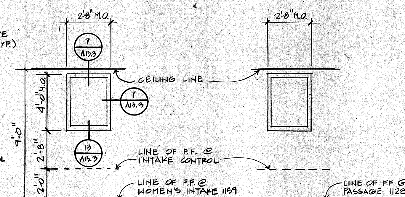
5 INTAKE 1130 ( 8\frac{3}{4}^{\circ} )
