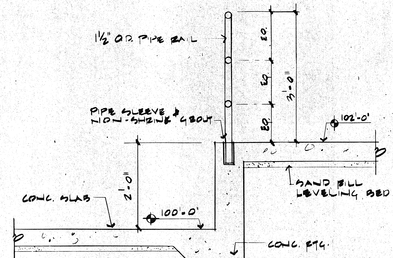
5 SECTION THRU RAISED PLATFORM SCALE: 1/4" = 1'-0"
