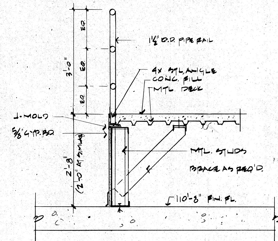
6 SECTION THRU RAISED FLOOR SCALE: 1/4" = 1'-0"
