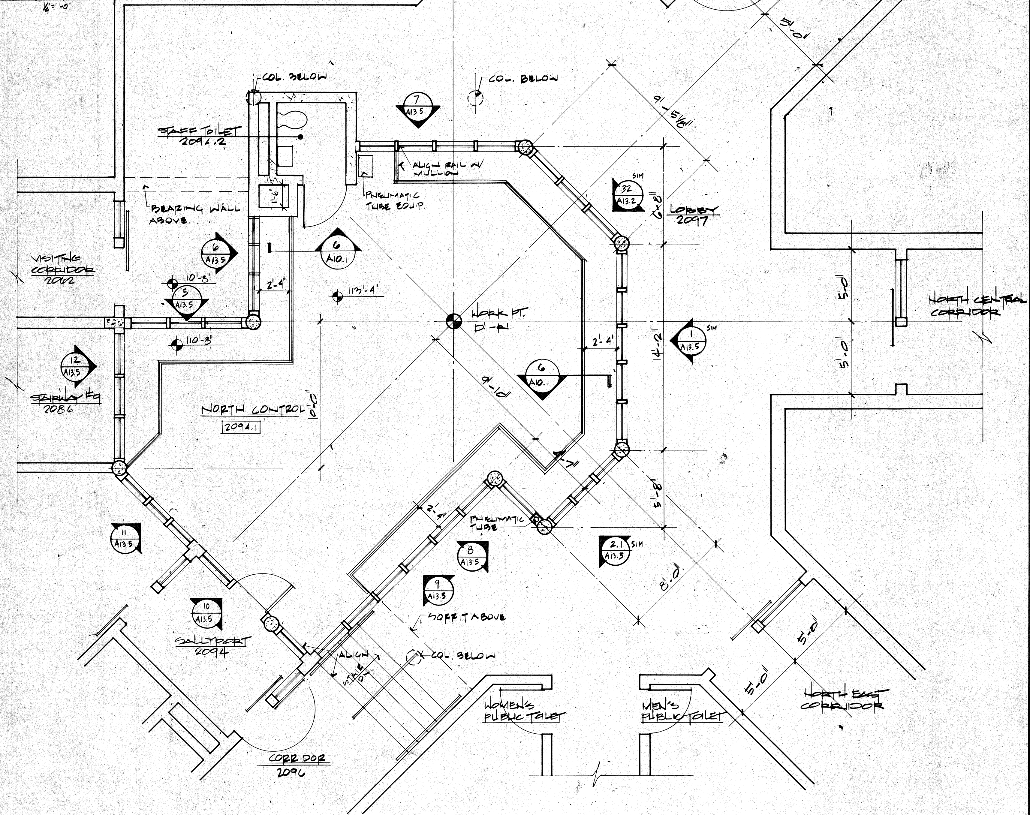
3 NORTH CONTROL ROOM - LEVEL 2 FLOOR PLAN SCALE: 1/4" = 1'-0"
