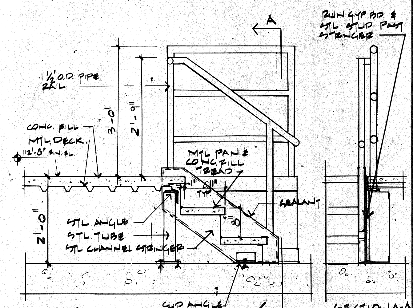
7 RAISED FLOOR STAIR SECTION SCALE: 1/4" = 1'-0"
