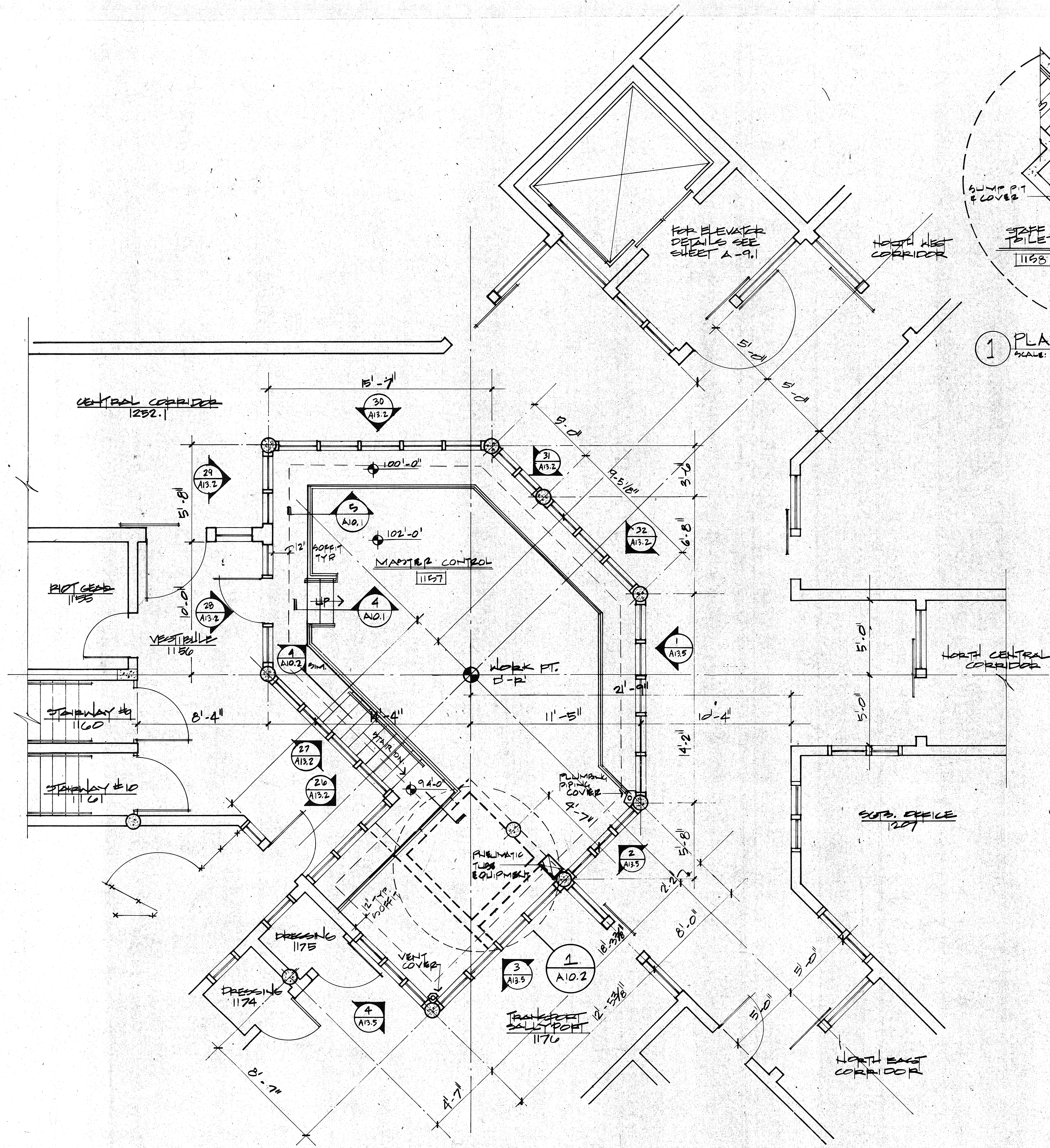
2 MASTER CONTROL ROOM - LEVEL 1 FLOOR PLAN SCALE: 1/4" = 1'-0"
